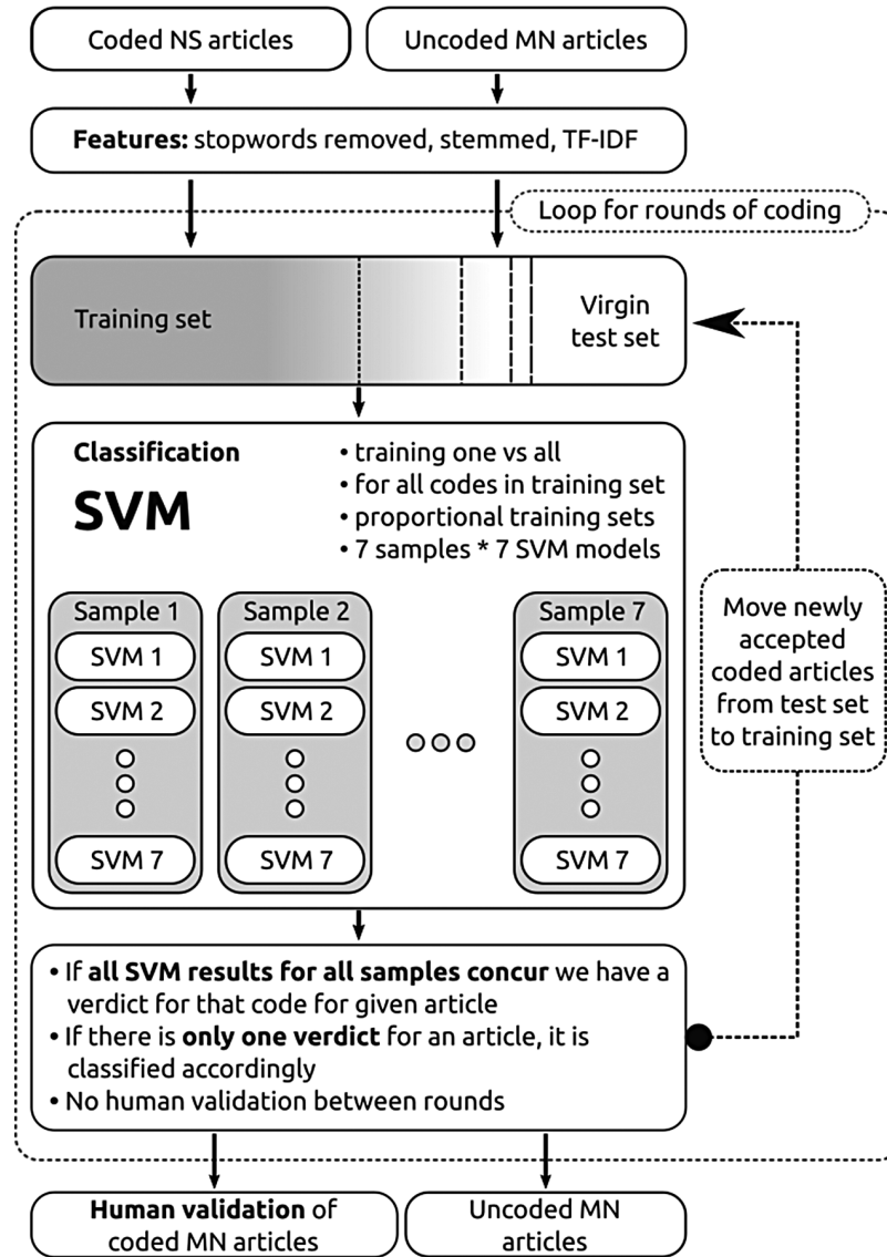
Figure 1. HBS in action: A coding process for a virgin corpus with in-process ensemble voting.
