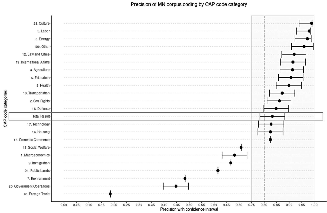
Figure 3. Precision of MN corpus coding by CAP major topic.
