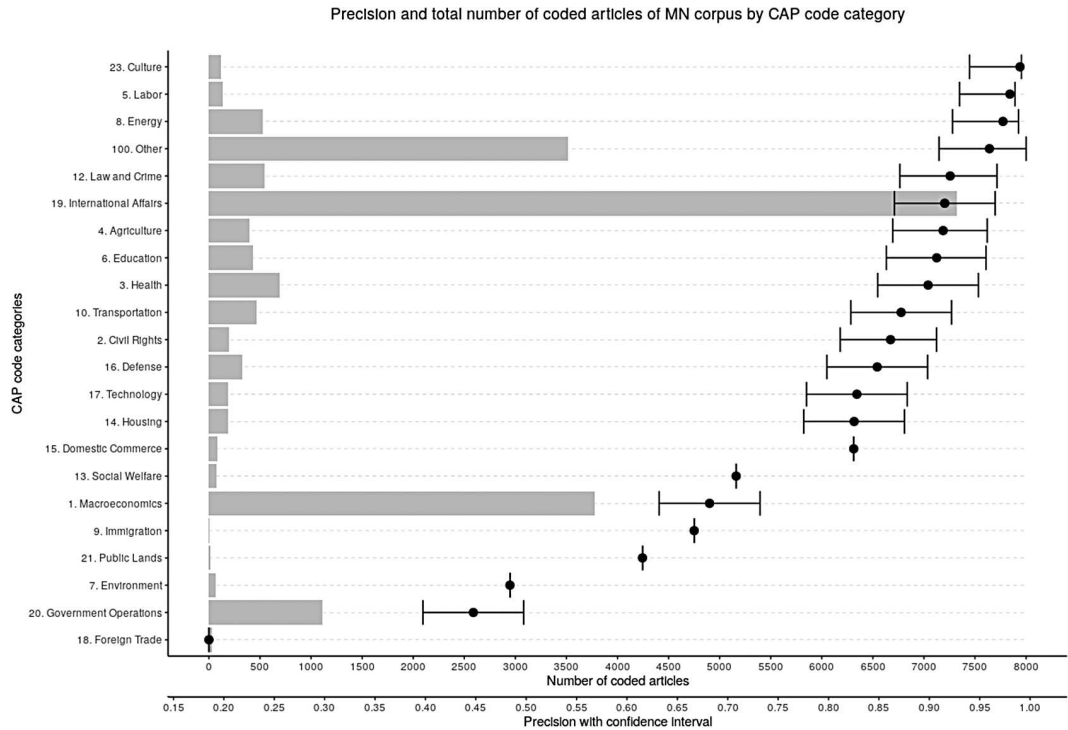
Figure 4. Precision of MN corpus coding by CAP major topic.
